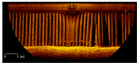
Quay wall inspection
